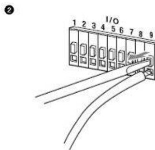
Figure 8-5 Remove cable
